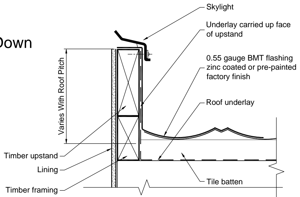
Section Across Scale 1:5
