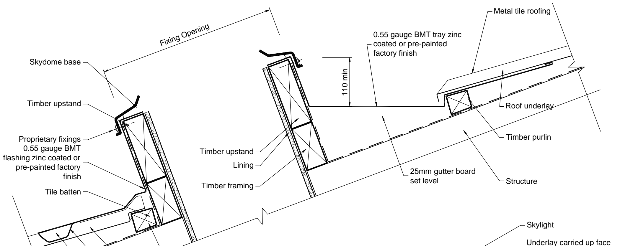
Section Down Scale 1:5
