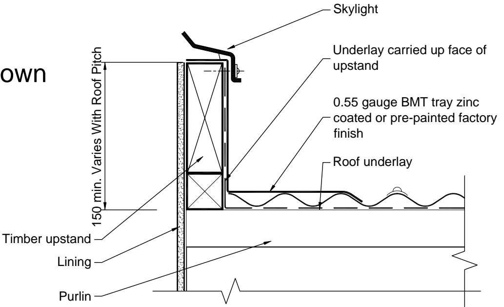
Section Across Scale 1:5
