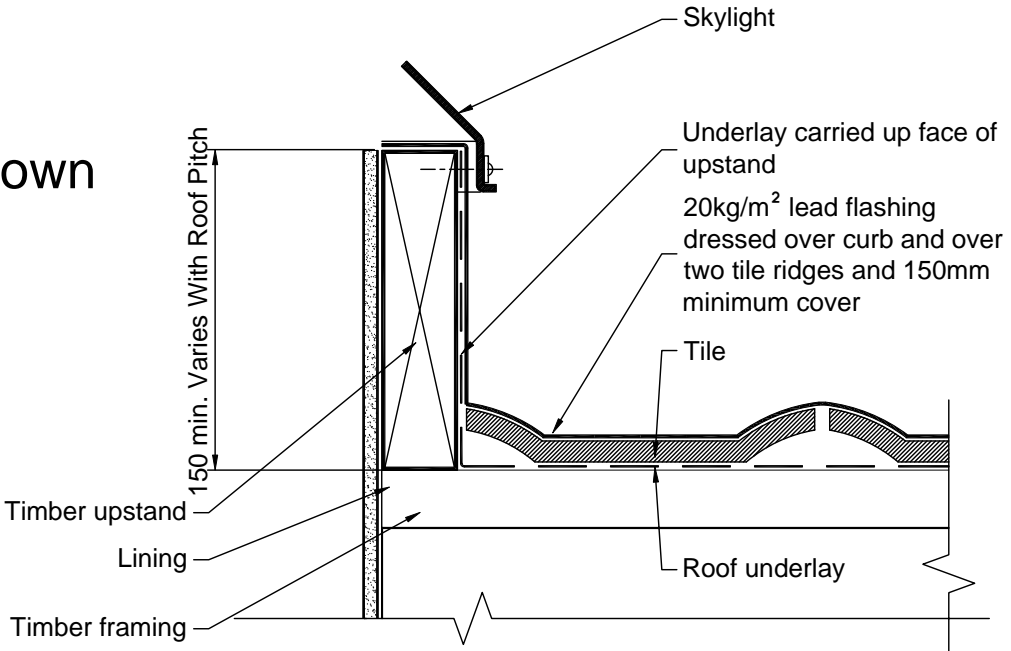
Section Across Scale 1:5
