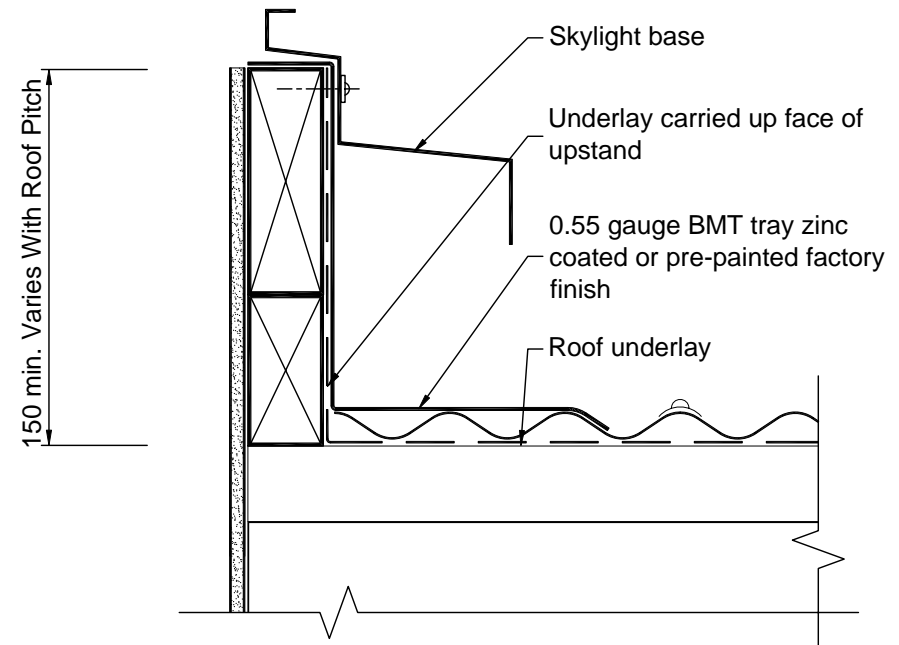
Section Across Scale 1:5
