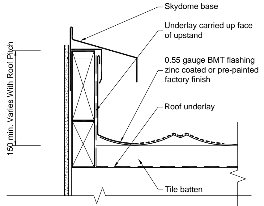
Section Across Scale 1:5
