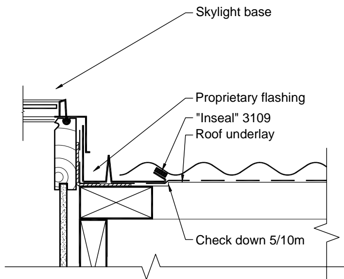
Section Across Scale 1:5
