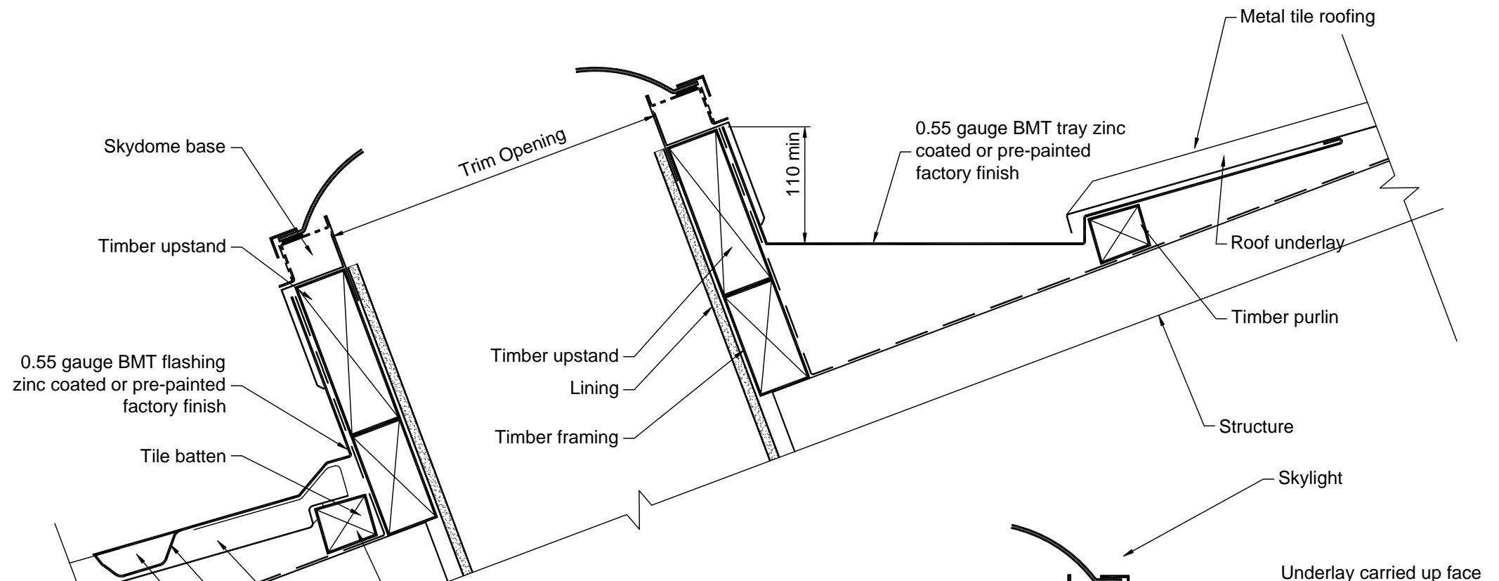
Section Down Scale 1:5
