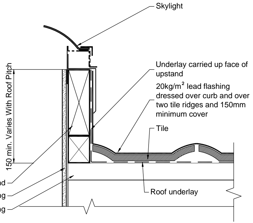
Section Across Scale 1:5
