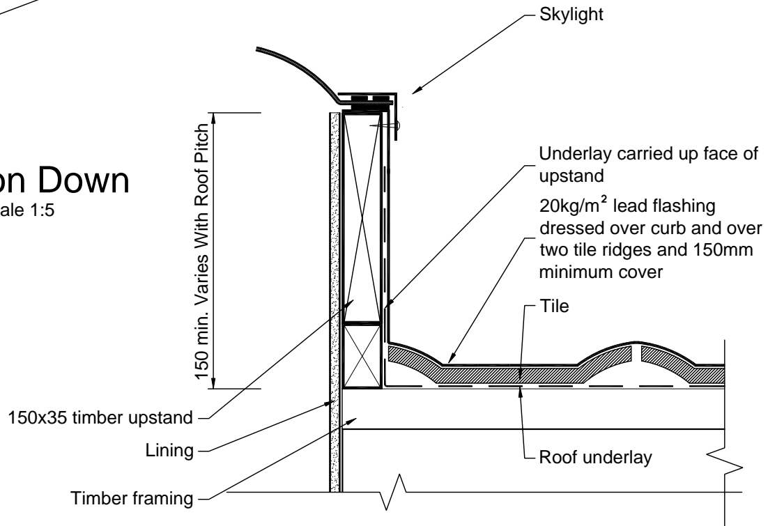
Section Across Scale 1:5
